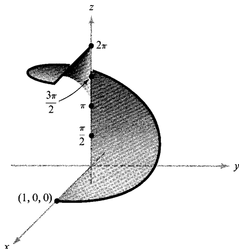
Figura 7.4.2 La helicoides x = r \cos \theta , y = r \sin \theta , z = \theta .
